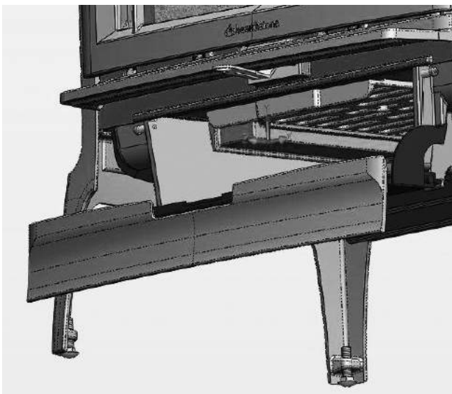
FIG. 5 - Grate handle
